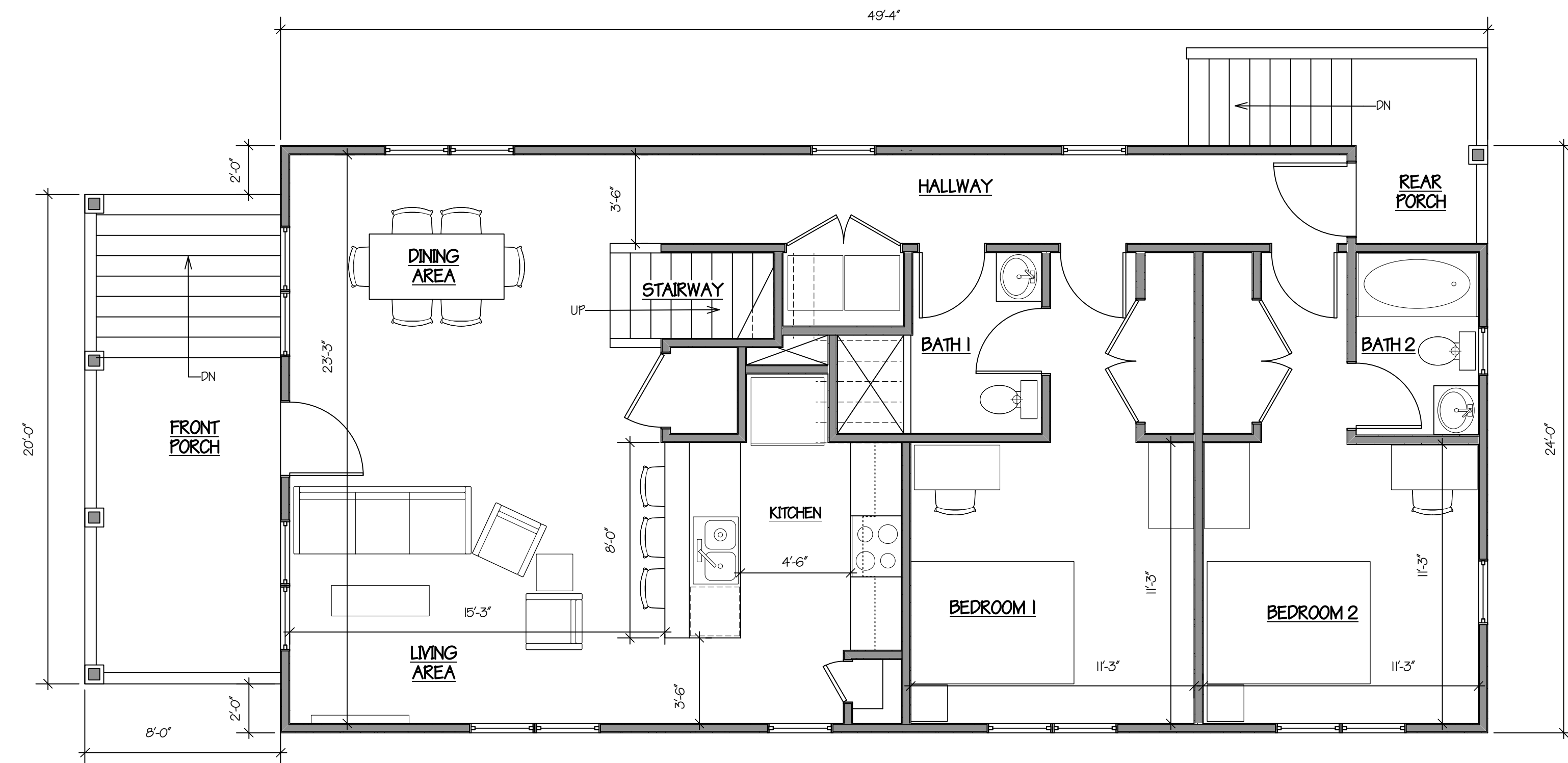
NEW HOUSE FIRST FLOOR PLAN 1/4"=1'-0" 0 10' 20' 30' 1163 S.F. FIRST FLOOR 672 S.F. SECOND FLOOR 1835 S.F. TOTAL FINISHED/CONDITIONED AREA
