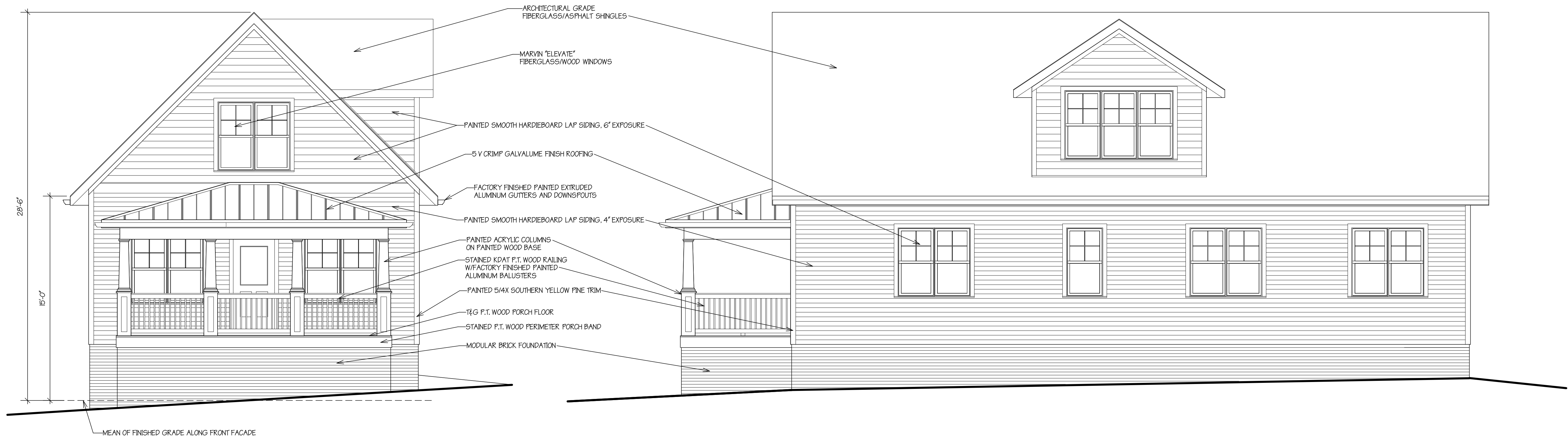
WEST / MALLETT STREET ELEVATION 1/4"=1'-0"
