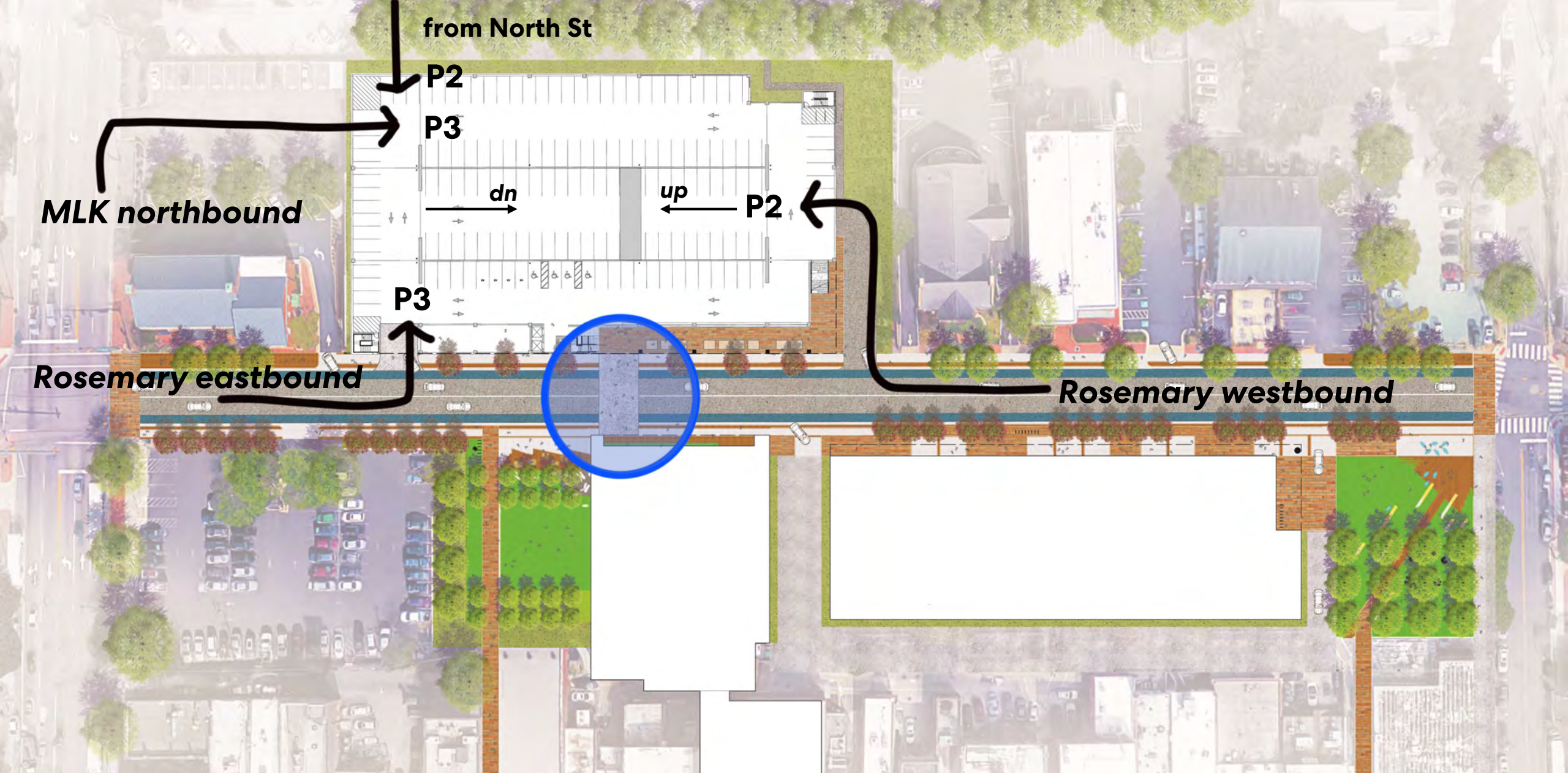
Morning Traffic Pattern with West Entrance
