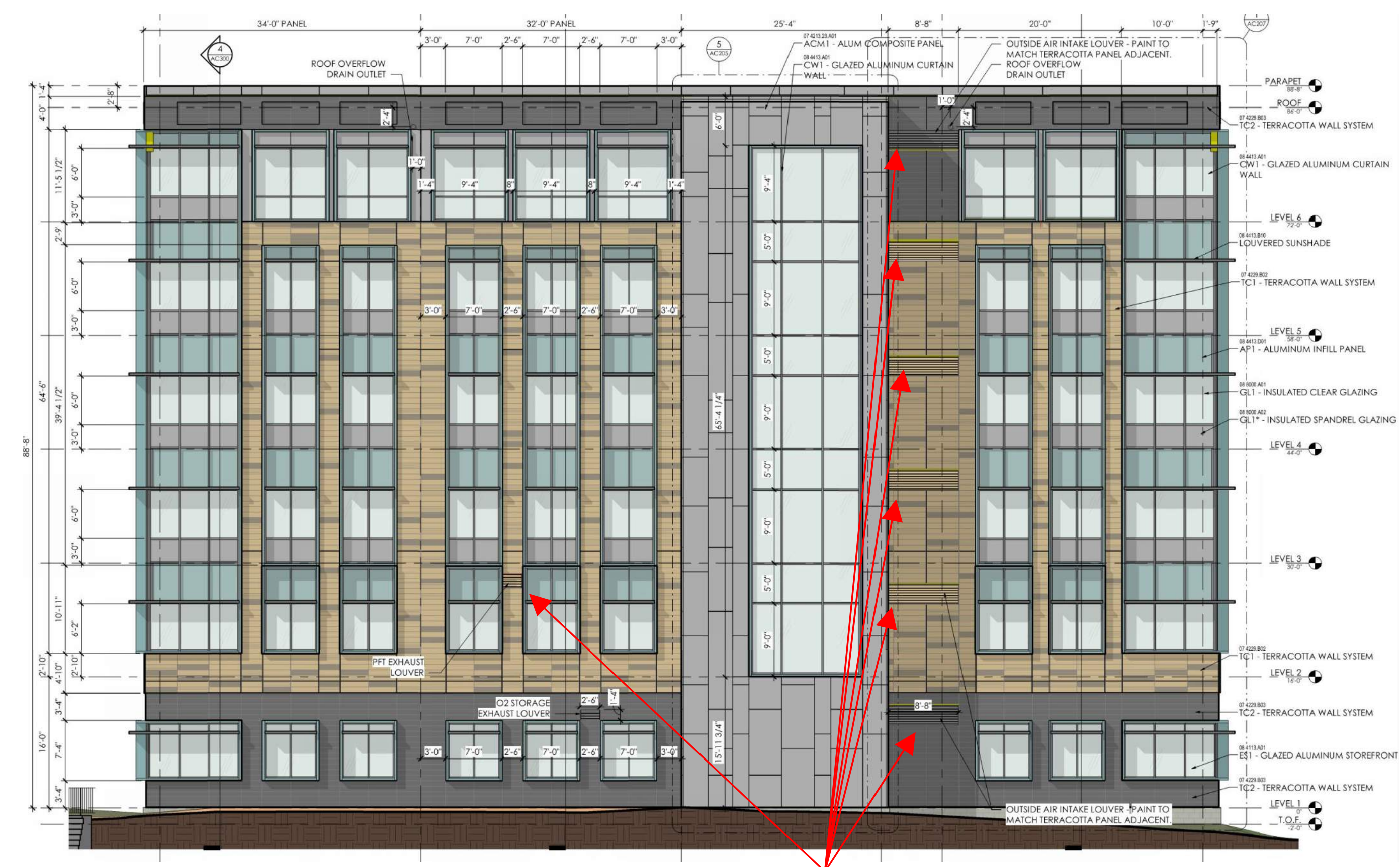
PROPOSED ORIGINAL WEST ELEVATION
