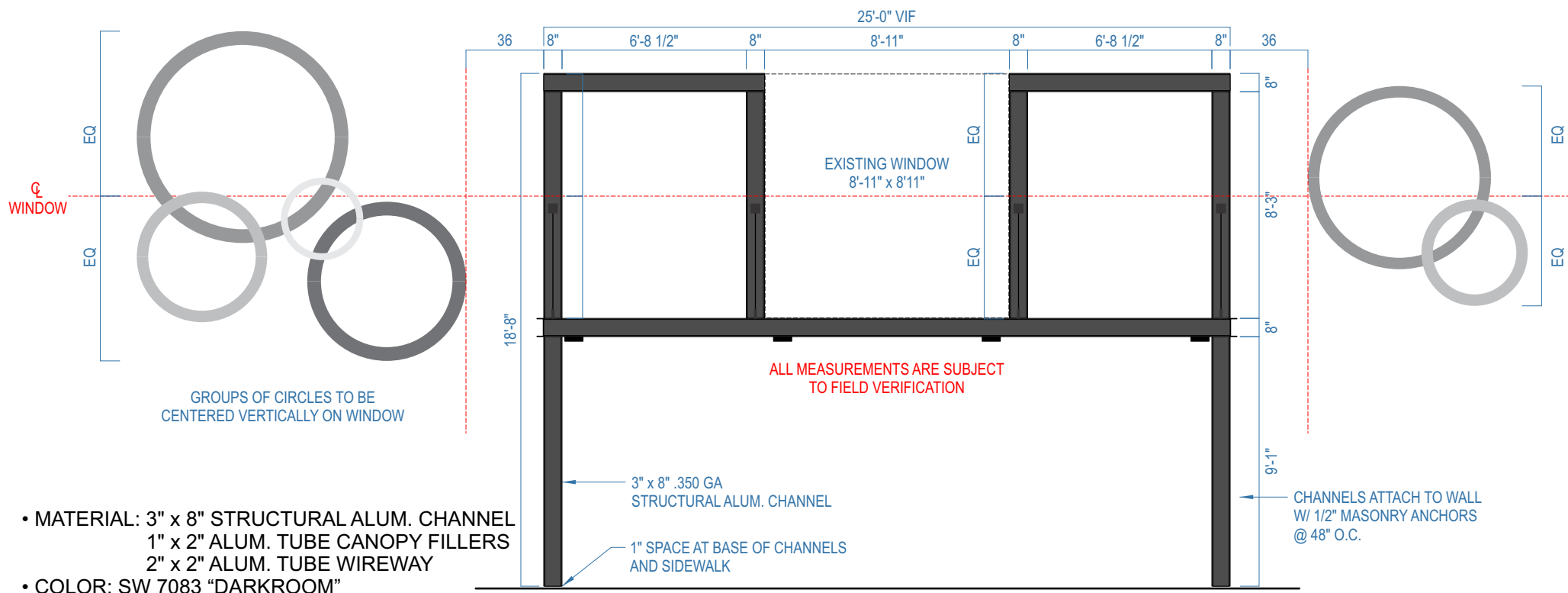
STOREFRONT CANOPY | ELEVATION Scale: 3/16" = 1'-0"
