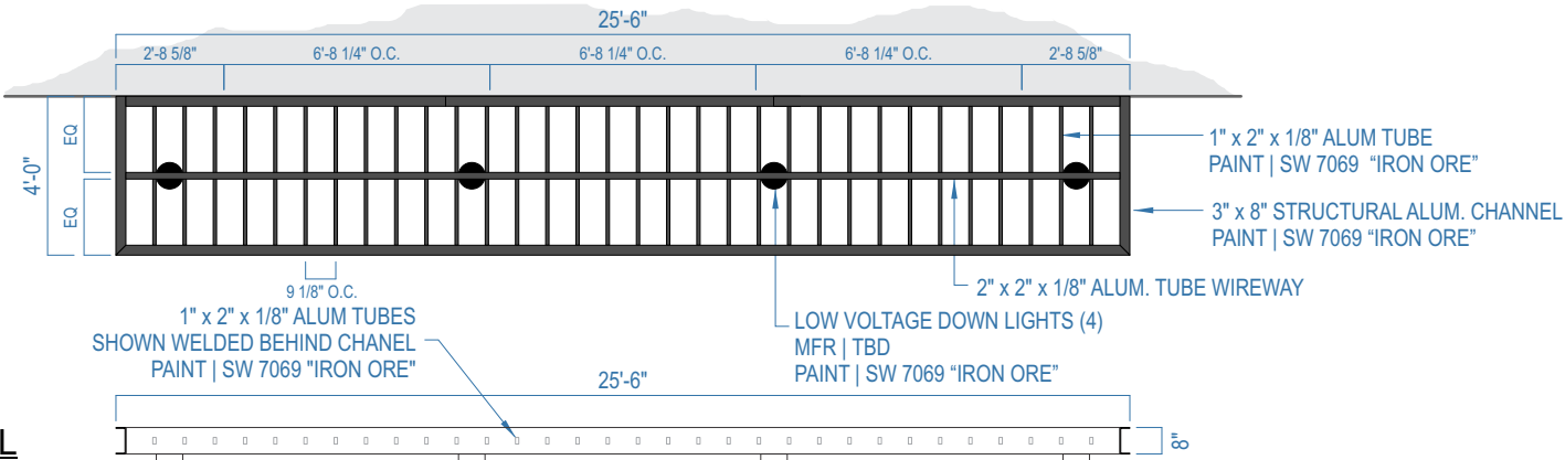
CANOPY | PLAN DETAIL Scale: 3/16" = 1'-0"
