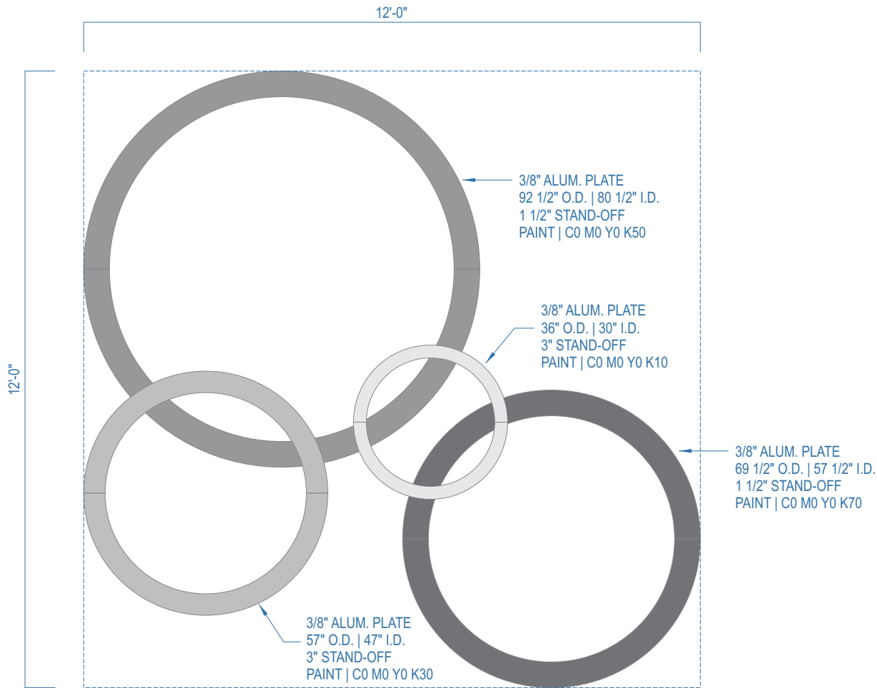
BACK LIT ACCENTS | FRONT VIEW Scale: 3/8" = 1'-0" QTY. REQ'D: ONE (1)
