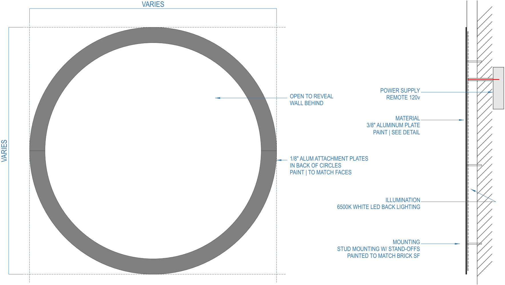
TYPICAL | BACK LIT ACCENT | FRONT VIEW Scale: NTS QTY. REQ'D: SIX (6)
