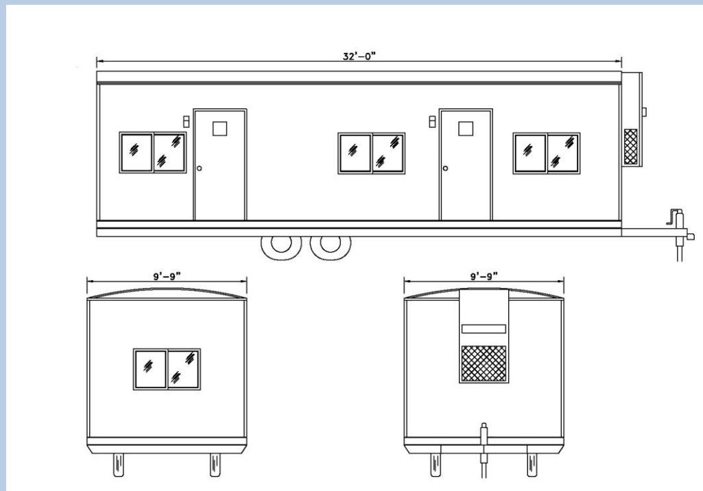
36 x 10' Office: Images and Elevations
