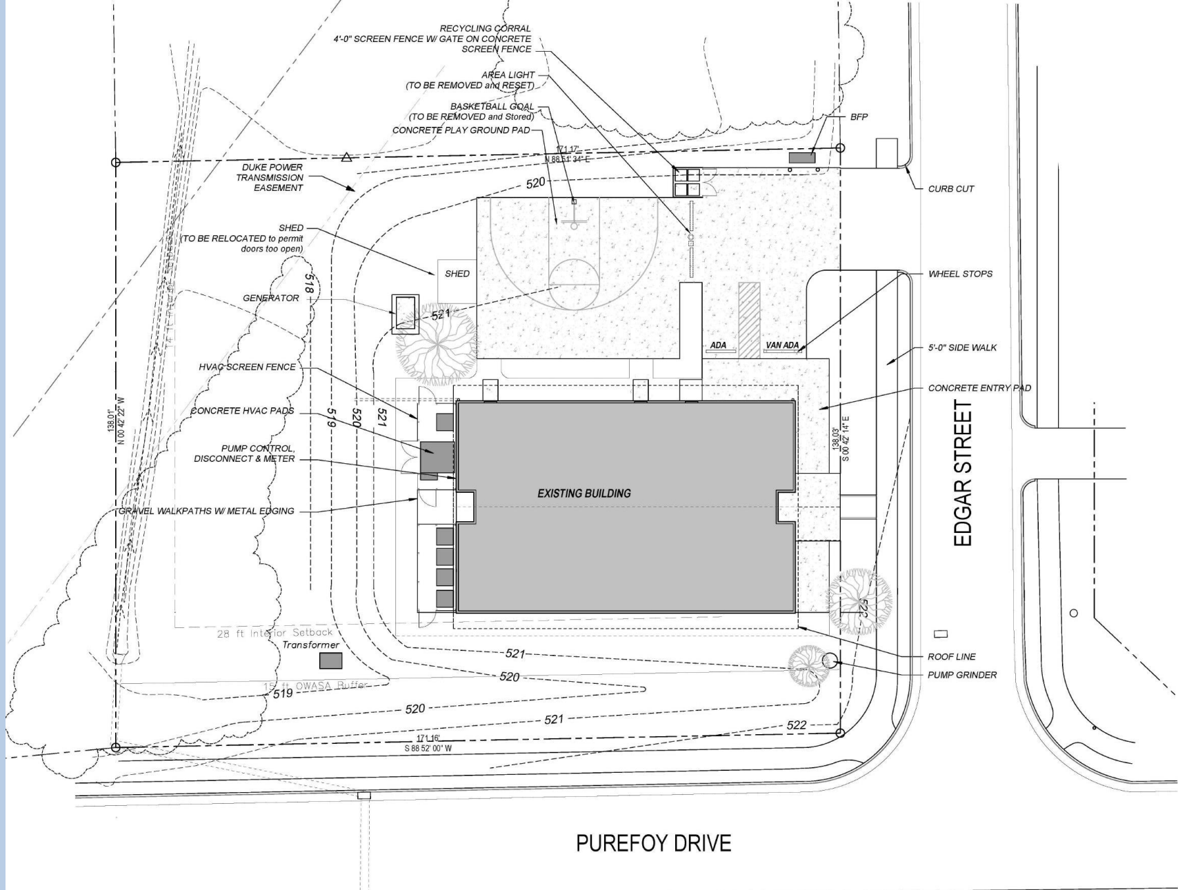
Existing Conditions - Plan View
