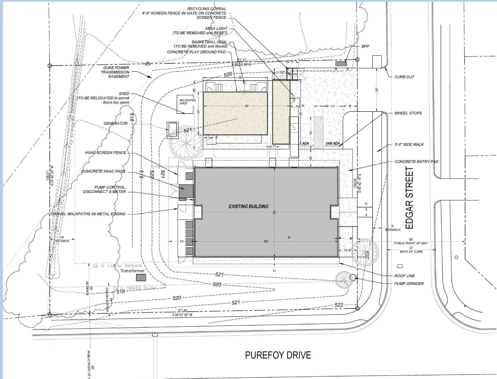
Proposed Classroom/Office Building – Plan View
