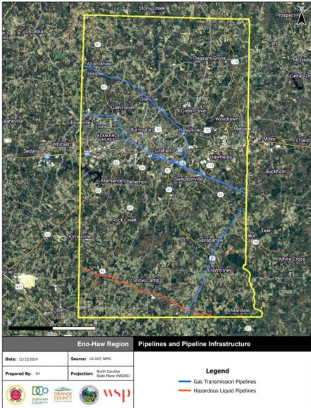
Figure 4.48 – Pipelines and Pipeline Infrastructure in Alamance County
