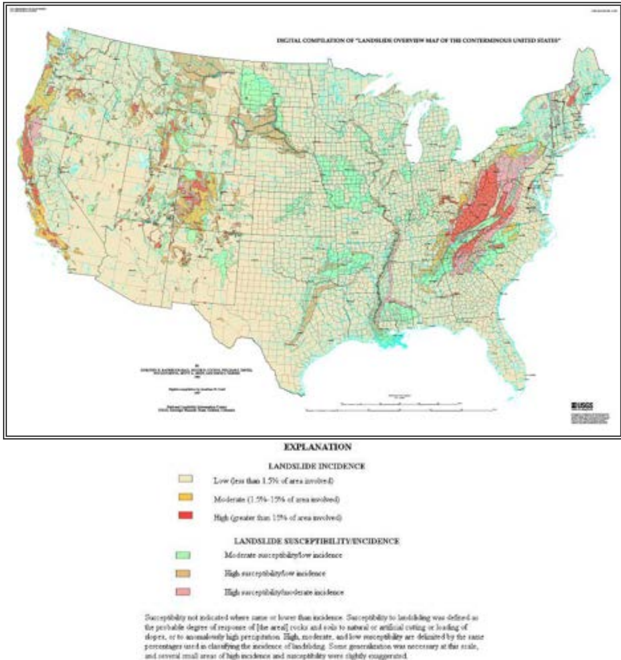
Figure 4.31 – Landslide Incidence and Susceptibility
