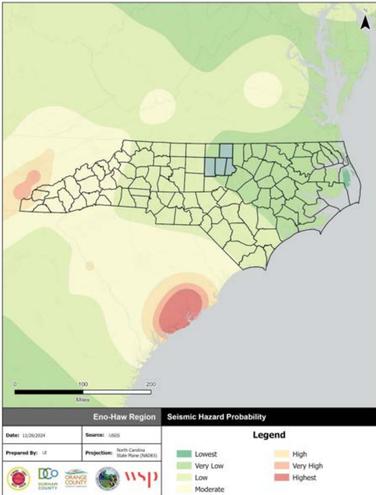
Figure 4.17 – Seismic Hazard Information for North Carolina
