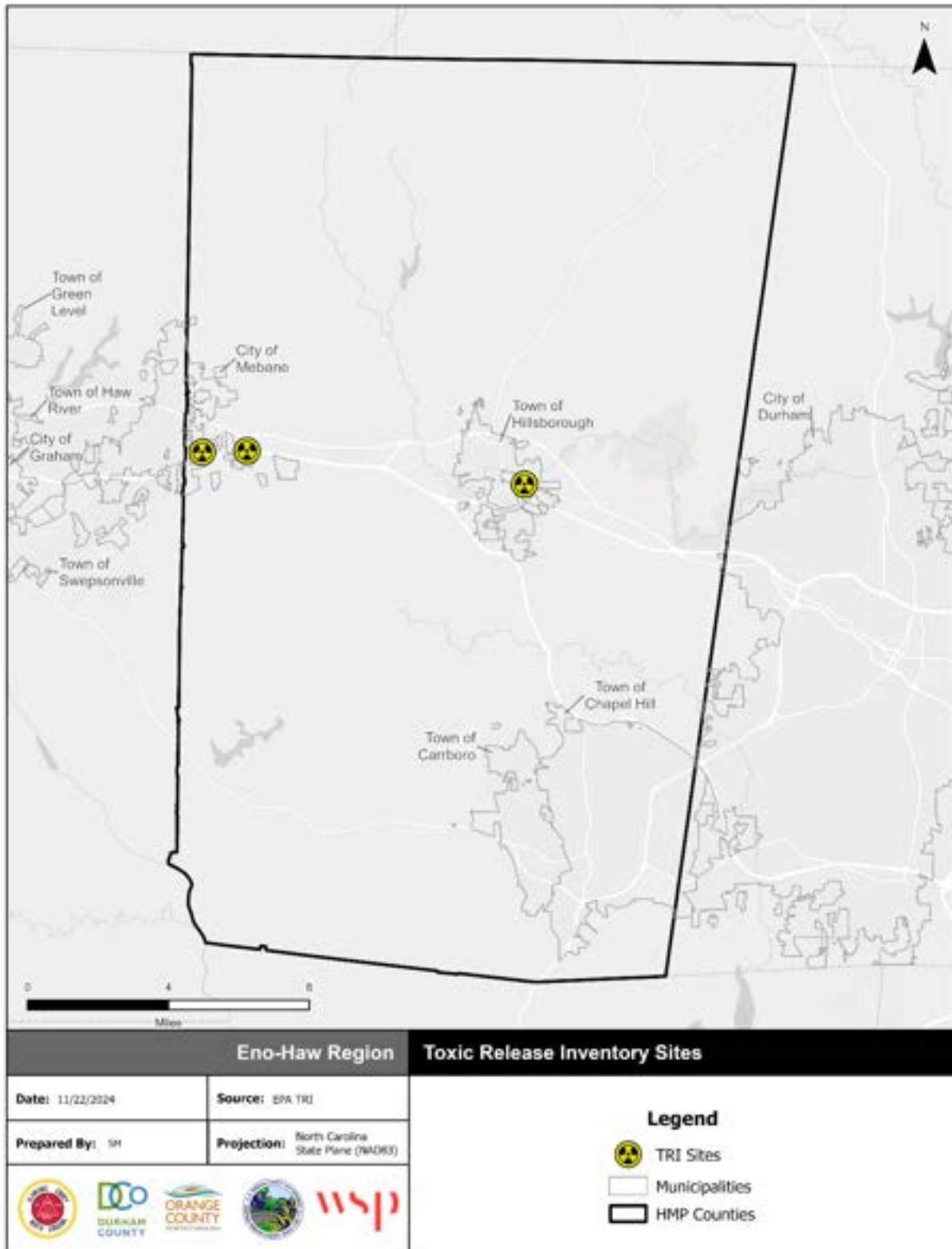
Figure 4.46 - Toxic Release Inventory Sites in Orange County
