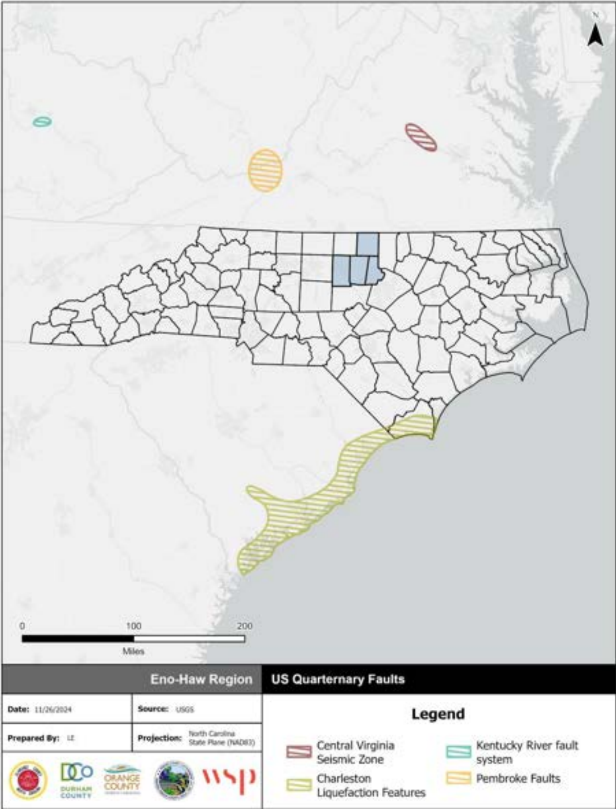
Figure 4.15 - US Quaternary Faults
