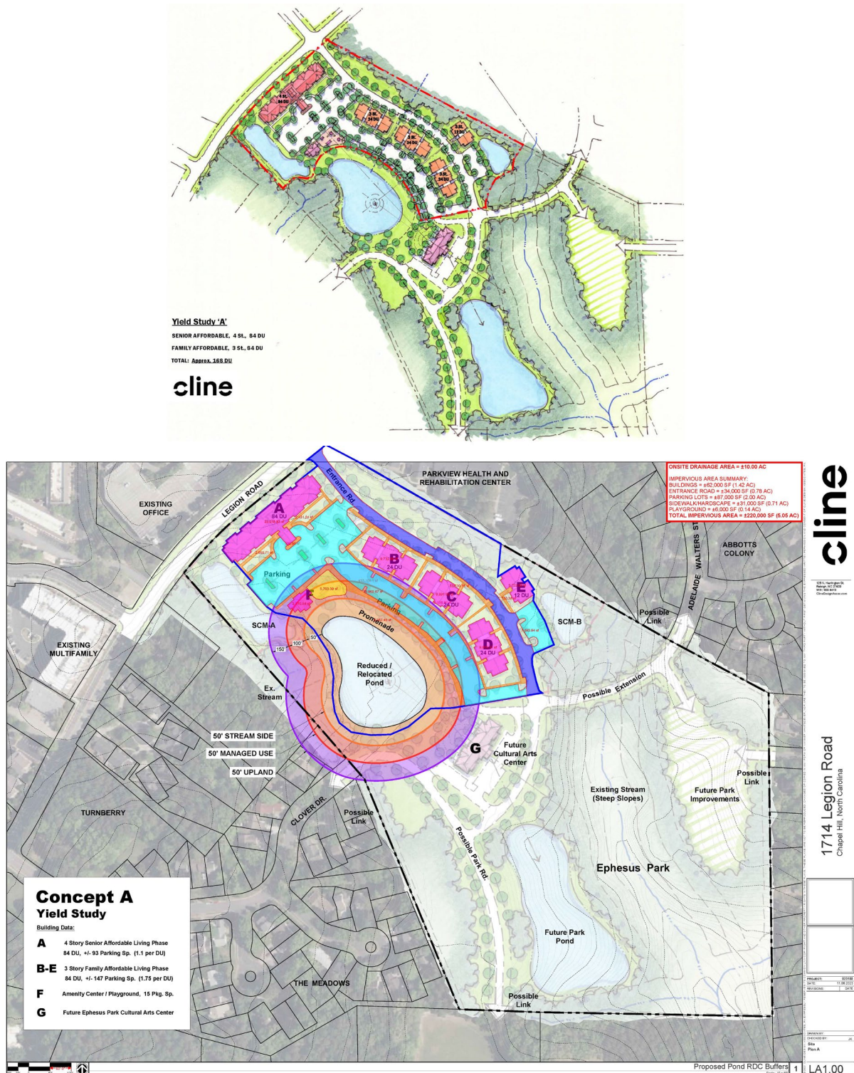
Figure 1-1. Option 1B: Reduce Pond Size – Preliminary Designs for Legion Pond in Relation to the Affordable Housing Project. (Designs from DHIC/clinc provided for reference only)
