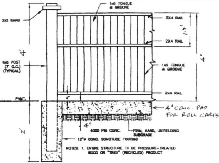
4" WOOD ROLL CART SCREEN NTS
