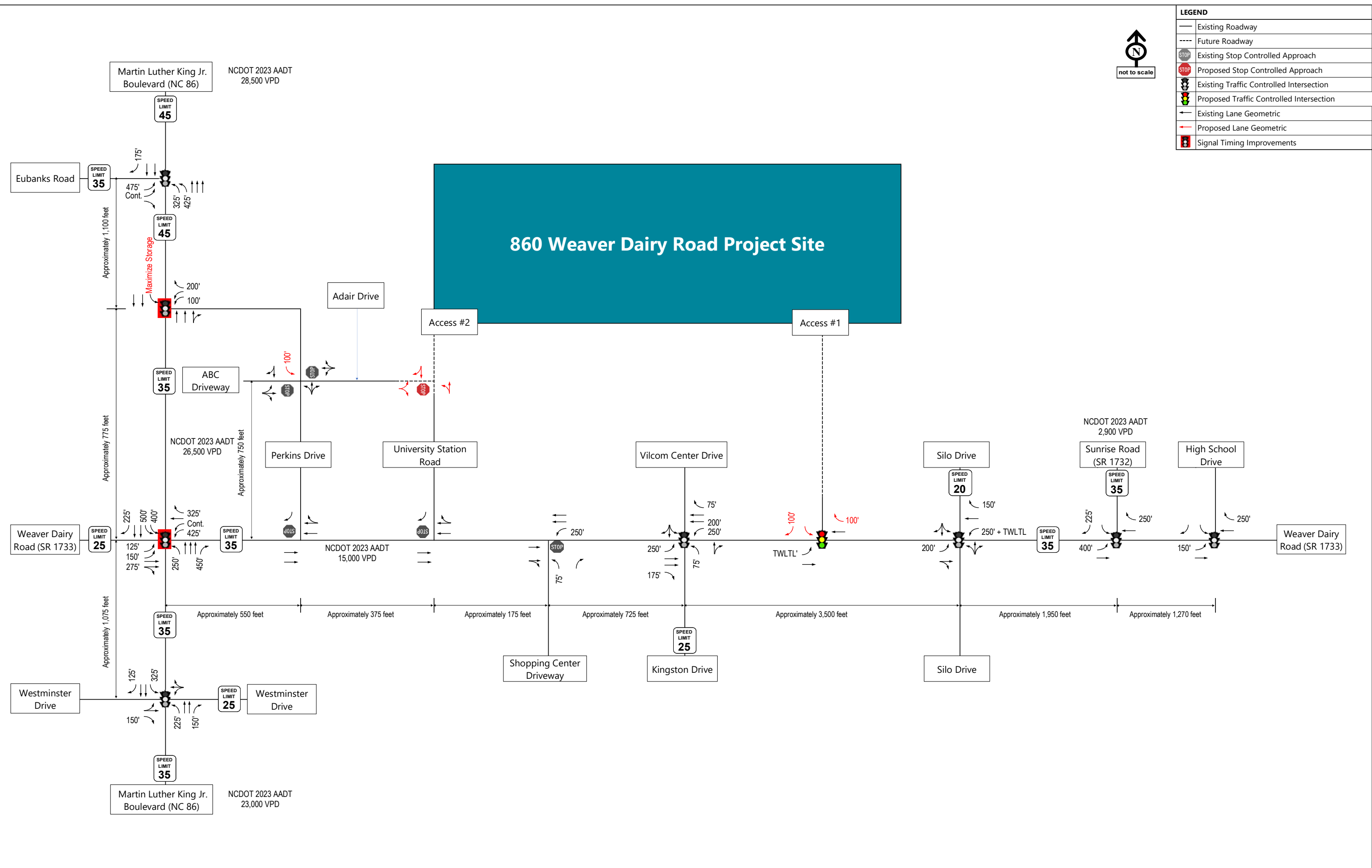
Figure 14 Build (2027) Lane Geometrics and Traffic Control – without STIP I-3306A
