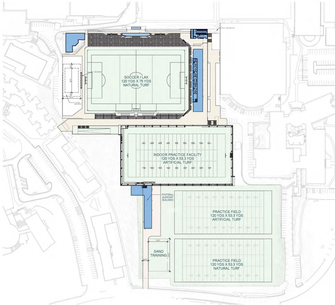
SITE PLAN
