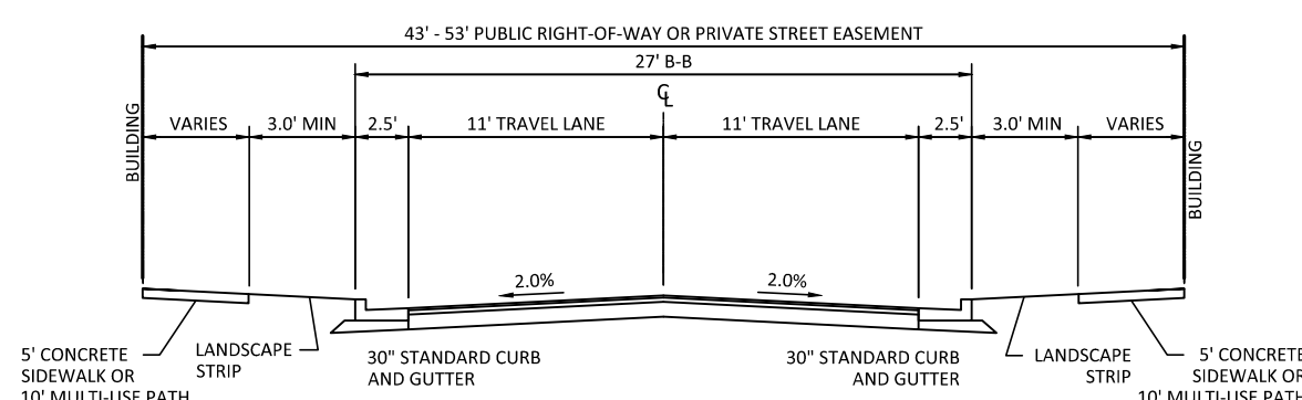
TYPICAL SECTION PRIVATE STREET WITH LANDSCAPE STRIP (43' - 53' R/W, 27' B-B)
