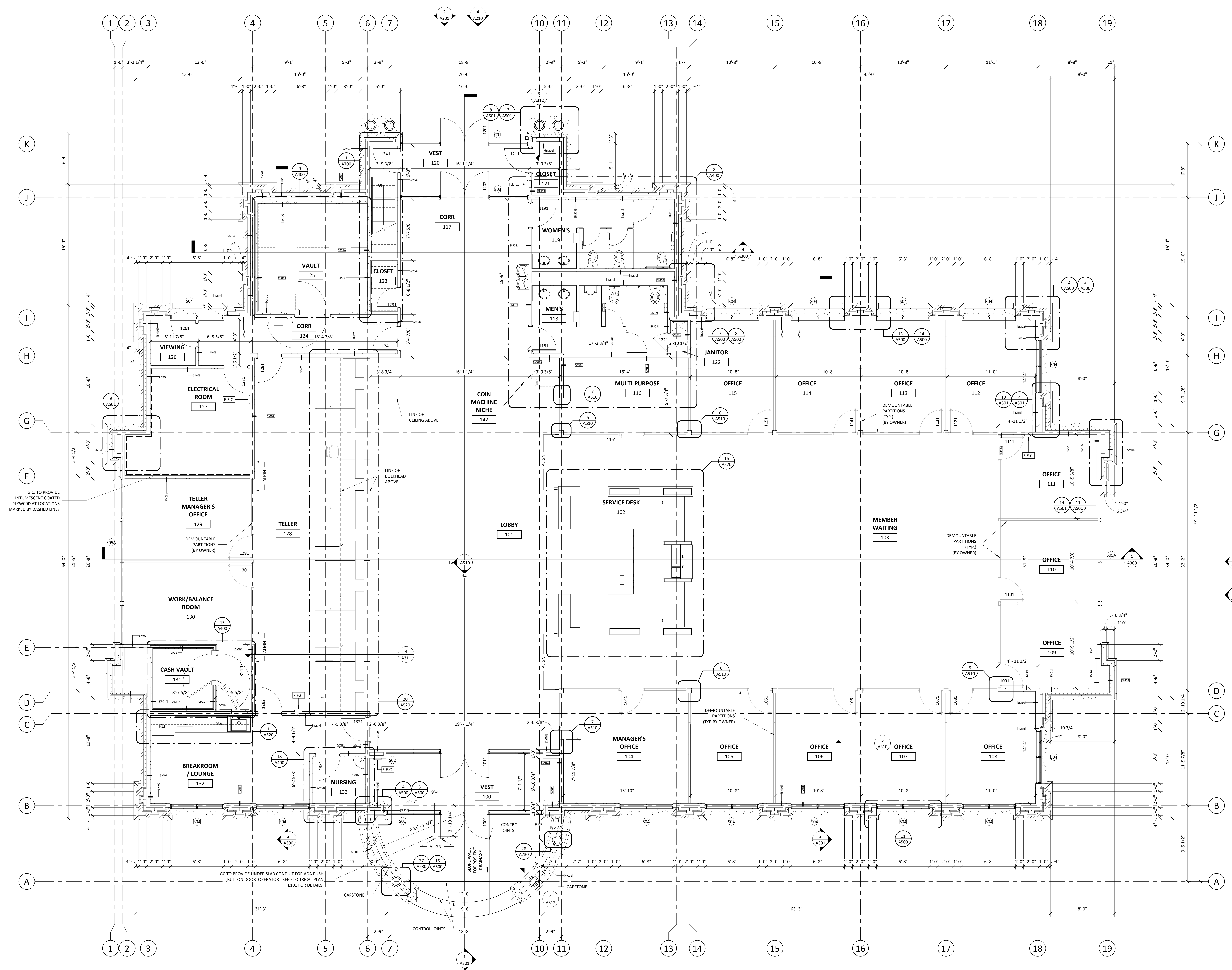
1 FIRST FLOOR PLAN 1/4" = 1'-0"
