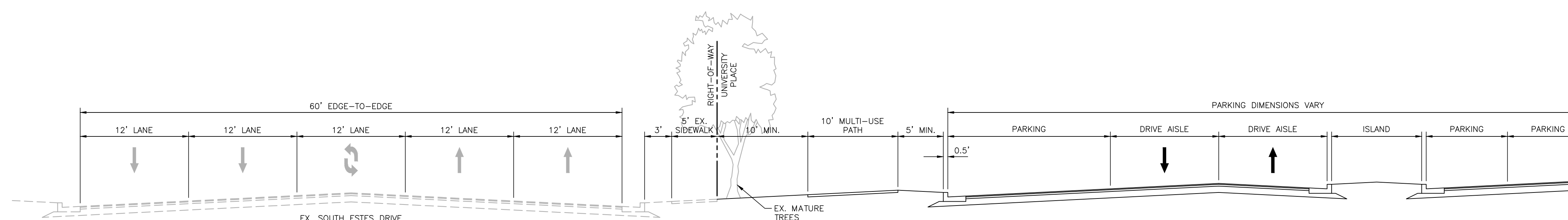
TYPICAL SECTION SOUTH ESTES DRIVE FRONTAGE
