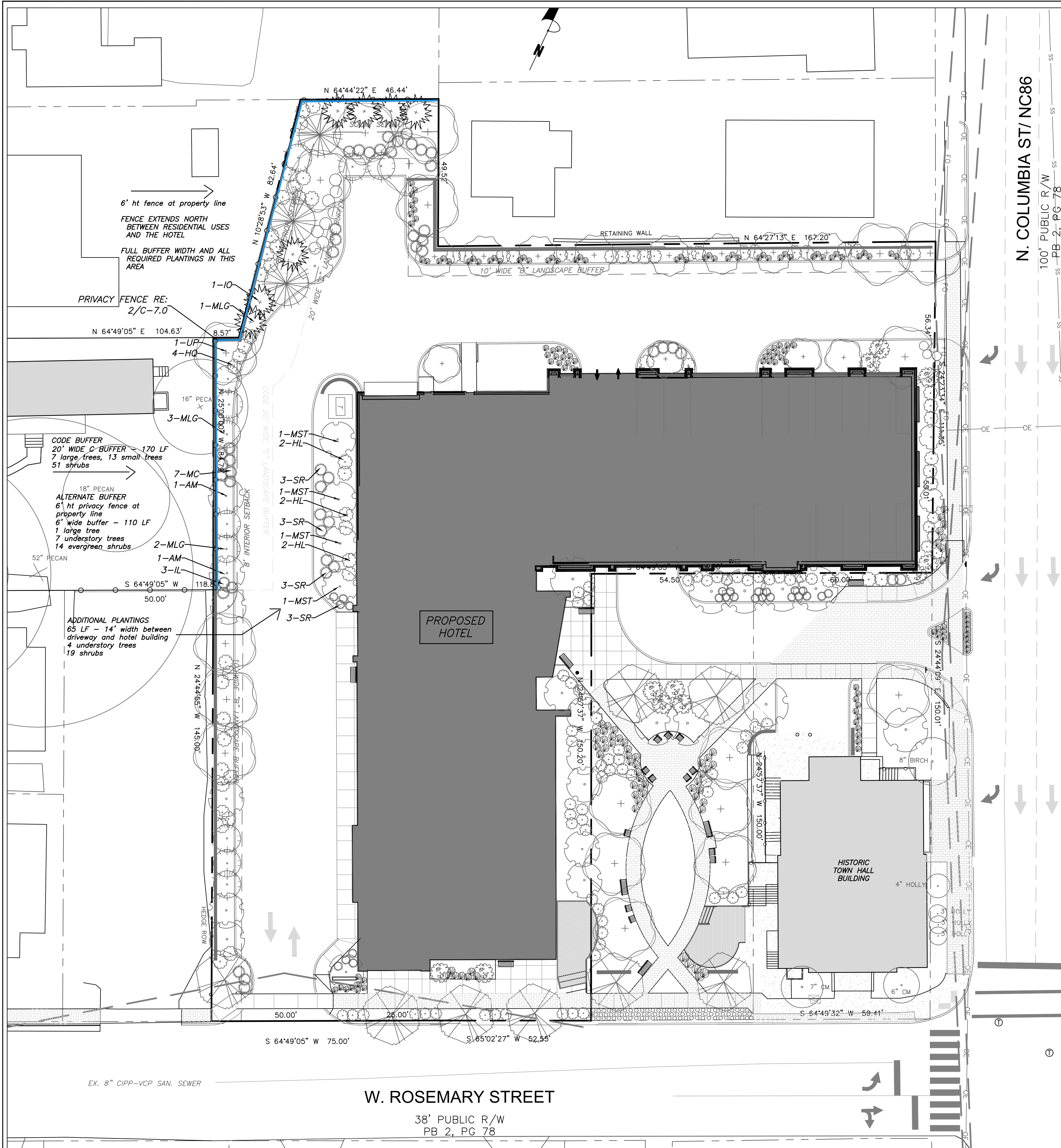
1 LANDSCAPE PLAN C-7.0
