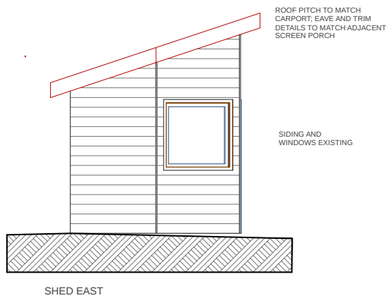
Modified/Proposed Side Shed Elevation
