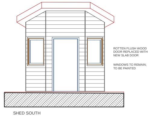
Modified/Proposed Front Shed Elevation
