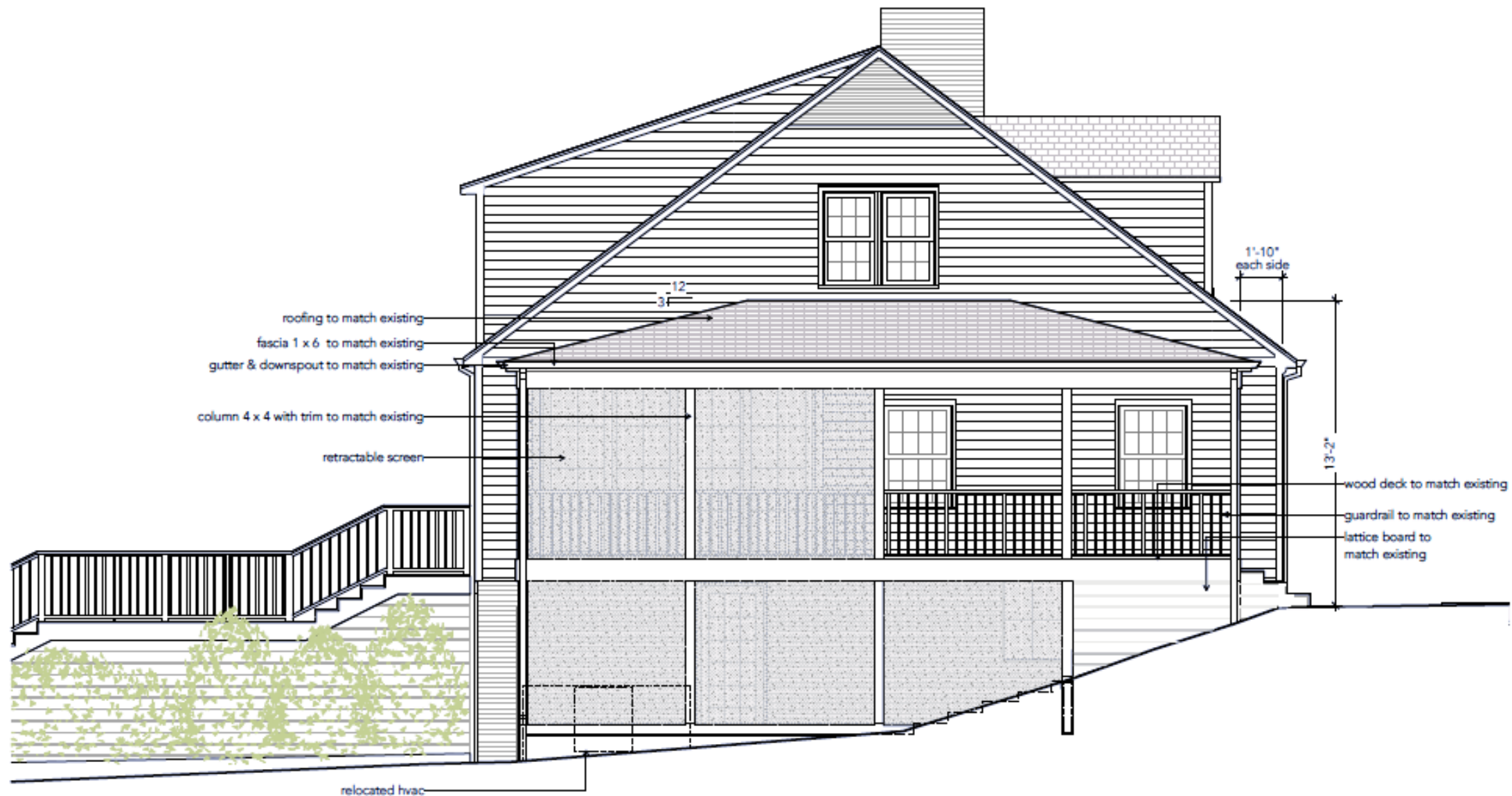
1 east elevation
