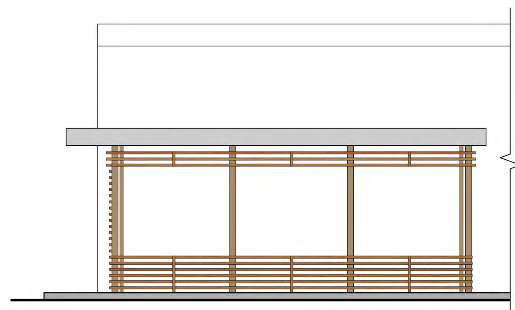
SOUTH ELEVATION ②A AT PATIO
