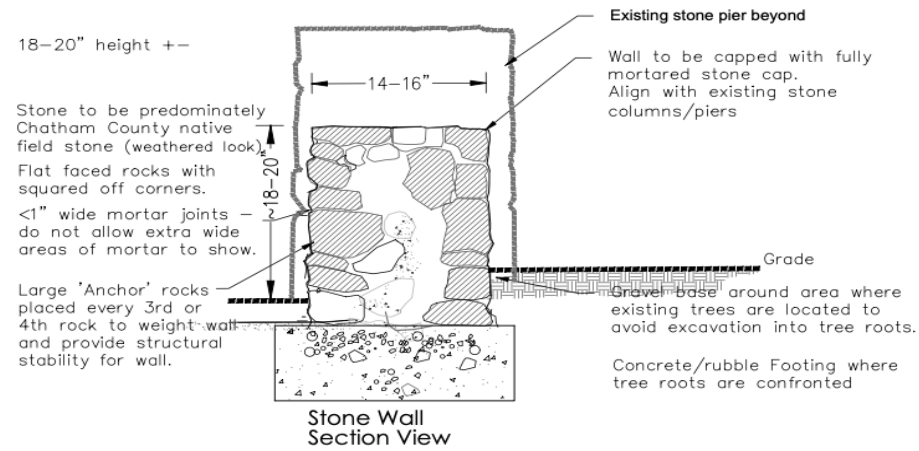
Example traditional stone wall using native Chatham stone
