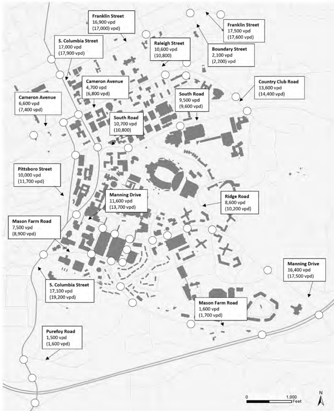
Figure 4-9: Future (2030) Average Daily Traffic Volumes
