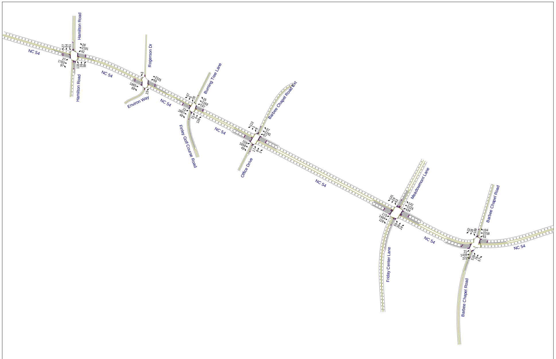
Figure 4-7d Future No-Build Year 2030 A.M. Peak Hour Turning Movement Volumes
