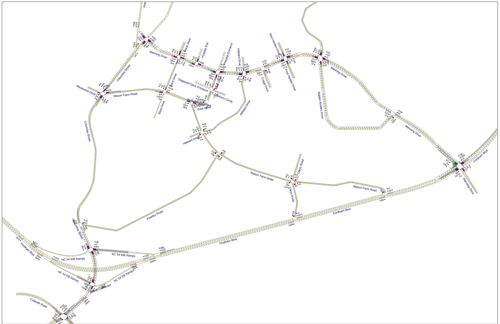
Figure 4-5b Year 2023 P.M. Peak Hour Turning Movement Volumes
